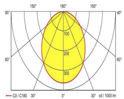
Aeroslim 18W Natural White
